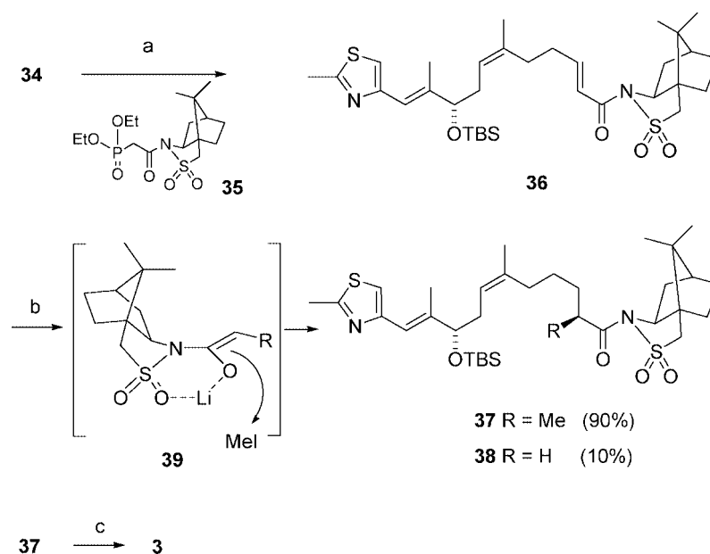
Scheme 6. Reagents and conditions: a) 35 , LiOH, THF, 0^{\circ}\text{C} , 0.5 h, 83%; b) i. L-selectride, THF, -78^{\circ}\text{C} , ii. LDA, MeI, HMPA, 16 h, room temp., 90%; c) DIBAL-H, -90^{\circ}\text{C} , DCM, 0.5 h, 90%.
