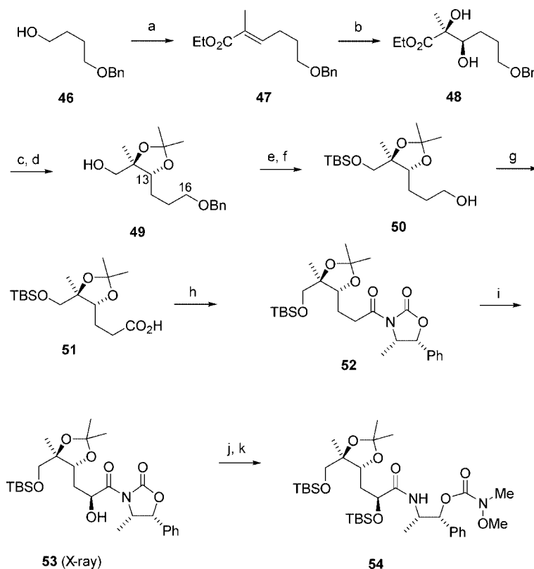
Scheme 9. Reagents and conditions: a) i. DMSO, oxalyl chloride, -78^{\circ}\text{C} , then diisopropylethylamine; ii. 1.1 equiv. ethyl 2-(triphenylphosphoranylidene)propionate, THF, 80^{\circ}\text{C} , 4 h, 84%; b) AD-mix \beta , \text{MeSO}_2\text{NH}_2 , t BuOH/ \text{H}_2\text{O} (1:1), room temp., 12 h, 96% (>98% ee ); c) (\text{MeO})_2\text{CMe}_2 , CSA, room temp., 38 h, 99%; d) 3 equiv. DIBAL-H, THF, 0^{\circ}\text{C} to room temp., 12 h, 94%; e) TBSCl, imidazole, DMF, room temp., 3 h, 99%; f) Pd/C (10%), ethyl acetate, \text{H}_2 (1 bar), room temp., 28 h, 92%; g) i. Dess–Martin periodinane, pyridine, \text{CH}_2\text{Cl}_2 , room temp., 4 h, ii. 5 equiv. \text{NaClO}_2 , \text{NaH}_2\text{PO}_4 , 2,3-dimethylbut-2-ene, t BuOH/ \text{H}_2\text{O} , room temp., 50 min, 93%; h) 1.1 equiv. \text{NET}_3 , 1.0 equiv. PivCl, \text{Et}_2\text{O} , -78 to 0^{\circ}\text{C} , 1 h, then Li salt of (4 S ,5 R )-4-methyl-5-phenyl-1,3-oxazolidinone, THF, -78 to 0^{\circ}\text{C} , 1 h, 76%. i) 1.4 equiv. NaHMDs, THF, -78^{\circ}\text{C} , 1 h, then 1.8 equiv. Davis oxaziridine, -92^{\circ}\text{C} , 5 min, then \text{NH}_4\text{Cl} , -92^{\circ}\text{C} to room temp., 10 min, 53% (> 96:4 dr ); j) TBSOTf, 2,6-lutidine, \text{CH}_2\text{Cl}_2 , room temp., 14 h, 95%; k) 4 equiv. \text{H}_2\text{N}(\text{OMe})\text{MeCl} , THF, \text{AlMe}_3 (2 M in toluene), room temp., 45 min, 74%.
