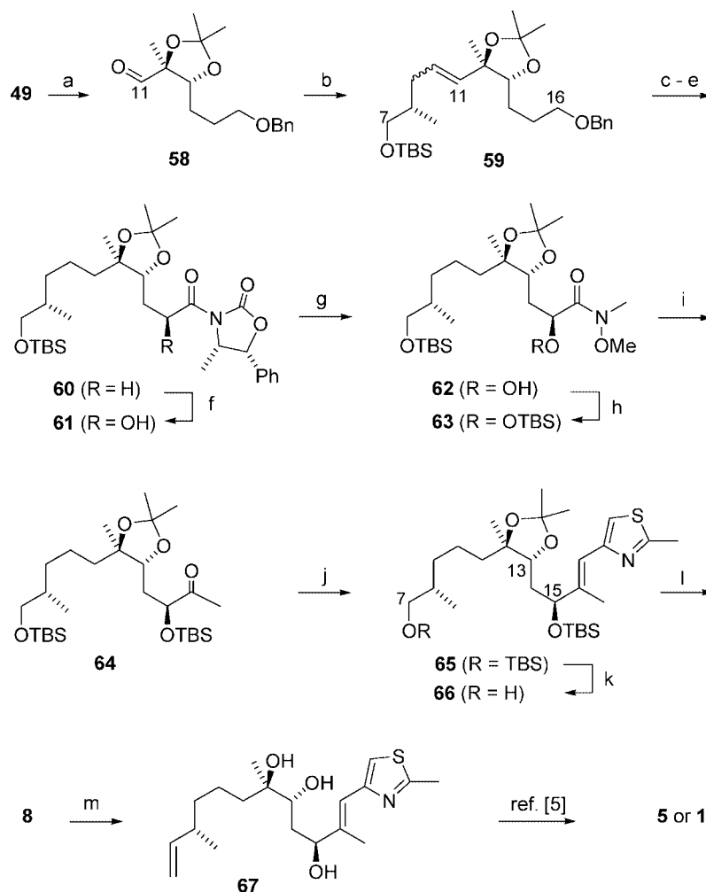
Scheme 11. Reagents and conditions: a) Dess–Martin periodinane, pyridine, CH 2 Cl 2 , room temp., 4 h; b) 1.1 equiv. NaHMDS, THF, 0 °C, 30 min, then 40 , 0 °C to room temp., 30 min, 87% over two steps; c) H 2 , Pd/Al 2 O 3 cat., EtOH, 3 bar, room temp., 36 h, 91%; d) 4 equiv. NaIO 4 , 0.05 equiv. RuCl 3 ·H 2 O, CCl 4 /MeCN/H 2 O (2:2:3), room temp., 80 min, 88%; e) 1.1 equiv. NEt 3 , 1.0 equiv. PivCl, Et 2 O, –78 to 0 °C, 1 h, then Li salt of (4 S ,5 R )-4-methyl-5-phenyl-1,3-oxazolidinone, THF, –78 to 0 °C, 1 h, 80%; f) 1.4 equiv. NaHMDS, THF, –78 °C, 1 h, then 1.8 equiv. Davis oxaziridine, –84 °C, 5 min, then NH 4 Cl, –84 °C to room temp., 10 min, 66% (> 96:4 dr ); g) 4 equiv. H 2 N(OMe)MeCl, 8 equiv. i PrMgCl, THF, –10 to 0 °C, 1 h, 94%; h) TBSOTf, 2,6-lutidine, CH 2 Cl 2 , 0 °C, 1 h, 97%; i) 1.1 equiv. MeLi, THF, –78 °C, 90 min, 91%; j) 5 equiv. 32 , 5 equiv. KHMDS, THF, –78 to 45 °C, 1 h, 98% ( E/Z , 30:1); k) 1 equiv. CSA, CH 2 Cl 2 /MeOH (1:1), 0 °C, 7 h, 97%; l) 1.3 equiv. Dess–Martin periodinane, pyridine, CH 2 Cl 2 , 0 °C, 4 h, 97%; m) i. triphenylmethylphosphonium iodide, n BuLi, hexane/THF; ii. TBAF (1 M in THF), THF, room temp., 5 h; iii. EtOH, 1 M HCl, 75%.
