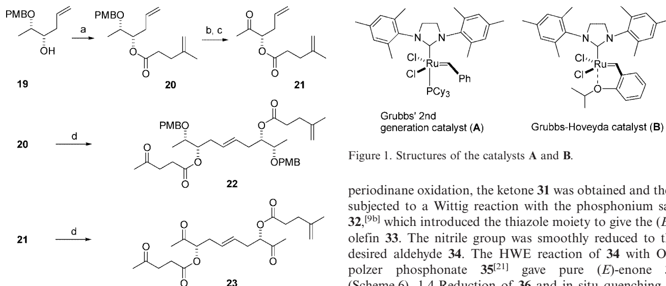
Scheme 4. Reagents and conditions: a) 4-methyl-4-pentenoic acid, EDCI, DMAP, DCM, 0 °C, 3 d, 83%; b) DDQ, DCM/H 2 O, (20:1), 0.5 h, 79%; c) DMP, DCM, NaHCO 3 , 4.5 h, 91%; d) A or B (15 mol-%), DCM, (2.6 mm), 40 °C, 16 h.
