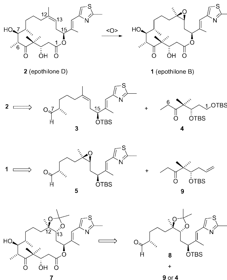
Scheme 1. Retrosynthetic considerations.
