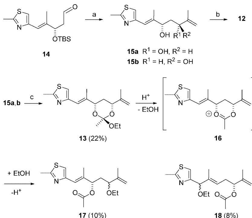
Scheme 3. Reagents and conditions: a) i. isopropenylmagnesium bromide, THF, 0 °C, 1 h, 97%; ii. TBAF, THF, room temp., 3 h, 97%; b) triphosgene, Et 3 N, pyridine, DCM, 1 h, -78 °C to room temp., 93%; c) amberlyst 15, triethyl orthoacetate (1 equiv.), xylene, 70 °C, 1 h, 40%.
