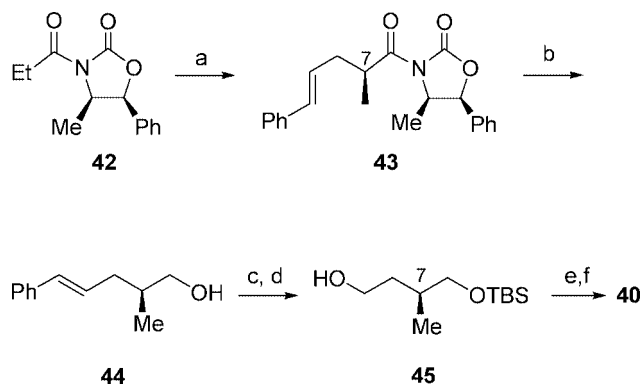
Scheme 8. Reagents and conditions: a) 1.1 equiv. NaHMDs, THF, then cinnamyl bromide, -78^{\circ}\text{C} to room temp., 4 h, 76% (> 96:4 dr ); b) 1.2 equiv. \text{LiBH}_4 , 1.1 equiv. \text{H}_2\text{O} , \text{Et}_2\text{O} , 0^{\circ}\text{C} to room temp., 2 h, 90%; c) TBSCl, imidazole, DMF, room temp., 3 h, 99%; d) NMO, \text{OsO}_4 (2 mol-%), THF/ t BuOH/ \text{H}_2\text{O} , room temp., 16 h; then \text{NaIO}_4 , THF/ \text{H}_2\text{O} , room temp. 3 h; then \text{NaBH}_4 , MeOH, 0^{\circ}\text{C} , 15 min, 89%; e) 3 equiv. imidazole, 1.5 equiv. \text{PPh}_3 , 1.5 equiv. \text{I}_2 , \text{Et}_2\text{O}/\text{MeCN} (3:1), 0^{\circ}\text{C} , 30 min; f) 1.5 equiv. \text{PPh}_3 , neat, 90^{\circ}\text{C} , 5 h, 76%.
