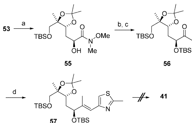
Scheme 10. Reagents and conditions: a) 4 equiv. H 2 N(OMe)MeCl, 4 equiv. i PrMgBr, THF, −10 °C to room temp., 2 h, 80%; b) TBSOTf, 2,6-lutidine, CH 2 Cl 2 , room temp., 14 h, 95%; c) 1.2 equiv. MeLi, THF, −78 °C, 2.5 h, 67%; d) 2, 2 equiv. KHMDS, THF, −78 to 45 °C, 1 h, 54% ( E/Z , 30:1).
