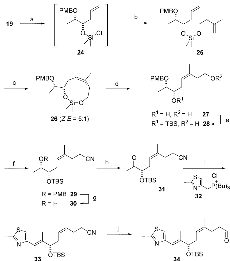
Scheme 5. Reagents and conditions: a) THF, -78^{\circ}\text{C} , n\text{BuLi} , then \text{SiMe}_2\text{Cl}_2 , room temp.; b) 3-methyl-3-butenol, DMAP, DMF, room temp., 24 h, 84%; c) A or B (15 mol-%), DCM (2.6 mM), 40^{\circ}\text{C} , 16 h, 98%; d) i. TBAF, THF, 12 h, 84%, ii. TBSOTf, DCM, 2,6-lutidine; e) HF/pyridine, 86%; f) \text{PPh}_3 , DEAD, 2-hydroxy-2-methylpropionitrile, \text{Et}_2\text{O} , 0^{\circ}\text{C} to room temp., 22 h, 89%; g) DDQ, DCM/ \text{H}_2\text{O} , (20:1), 0.5 h, 91%; h) (\text{COCl})_2 , DCM, DMSO, \text{Et}_3\text{N} , -78^{\circ}\text{C} , 1 h, 95%; i) 32 , n\text{BuLi} , THF, 0^{\circ}\text{C} , 1 h, then 31 , -78^{\circ}\text{C} to -60^{\circ}\text{C} , 1 h, 94%; j) DIBAL-H, toluene, -78^{\circ}\text{C} , 2 h, 84%.
