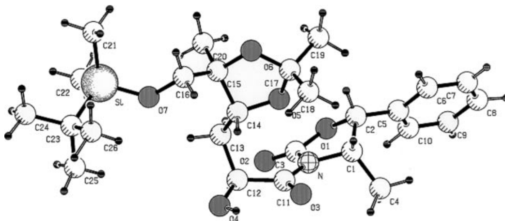
Figure 2. Crystal structure of compound 53 .
