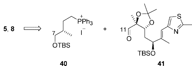
Scheme 7. Retrosynthesis of Northern fragments 5 and 8.
