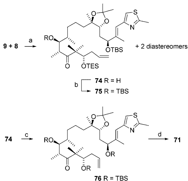
Scheme 13. Reagents and conditions: a) 9 , LDA, THF, -78^{\circ}\text{C} , 45 min, then 8 , 20 min, 70% (6:1:1); b) TBSOTf, 2,6-lutidine, \text{CH}_2\text{Cl}_2 , room temp., 3 h; c) TBAF, THF, -18^{\circ}\text{C} , 80 min; then TBSOTf, 2,6-lutidine, \text{CH}_2\text{Cl}_2 , room temp., 3 h, 81% over 3 steps; d) \text{OsO}_4 (0.05 equiv.), NMO (1 equiv.), THF, t BuOH, room temp., 14 h; then \text{NaIO}_4 , \text{H}_2\text{O} , room temp., 2 h, then 5 equiv. \text{NaClO}_2 , \text{NaH}_2\text{PO}_4 , 2,3-dimethylbut-2-ene, t BuOH/ \text{H}_2\text{O} , room temp., 50 min, 71% over 3 steps.
