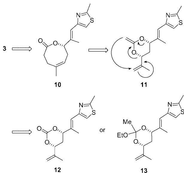
Scheme 2. Retrosynthesis of Northern fragment 3.
