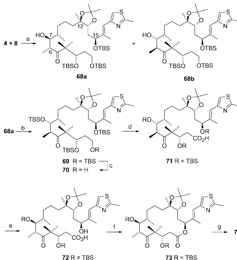
Scheme 12. Reagents and conditions: a) 4 , LDA, THF, -78^{\circ}\text{C} , 45 min, then 8 , 50 min, 73 % ( 68a/68b = 6:1); b) TBSOTf, 2,6-lutidine, \text{CH}_2\text{Cl}_2 , 0^{\circ}\text{C} , 12 h, 93%; c) CSA, \text{CH}_2\text{Cl}_2/\text{MeOH} (1:1), 0^{\circ}\text{C} , 8 h, 84%; d) i. 1.3 equiv. Dess–Martin periodinane, pyridine, \text{CH}_2\text{Cl}_2 , 0^{\circ}\text{C} , 2 h, ii. 5 equiv. \text{NaClO}_2 , \text{NaH}_2\text{PO}_4 , 2,3-dimethylbut-2-ene, t\text{BuOH}/\text{H}_2\text{O} , room temp., 50 min, 93%; e) 7 equiv. TBAF, THF, room temp., 12 h 82%; f) 1.2 equiv. 2,4,6-trichlorobenzoyl chloride, 2 equiv. \text{NEt}_3 , toluene, room temp., 2 h, then add to a solution of 10 equiv. DMAP in toluene, 110^{\circ}\text{C} , 3 h, 50% over two steps; g) 15% \text{CF}_3\text{CO}_2\text{H} in \text{CH}_2\text{Cl}_2 , -18 to 0^{\circ}\text{C} , 6 h, 80%.
